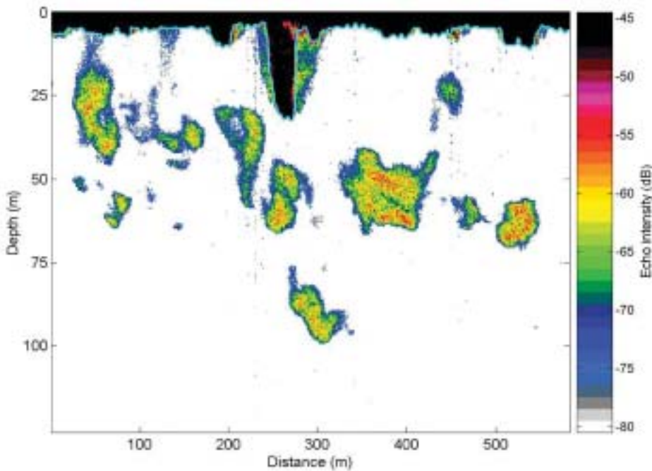
Figure 23. An echogram from the 38 kHz Simrad EK500 upward-looking echo sounder installed on Autosub for a cruise in February 2001. The vehicle was travelling at a depth of 150 m. The color scale represents echo intensity, where the patches in mid water were due to swarms of krill. The black trace represents echoes from the underside of the sea ice, from which ice draft can be estimated. For the Autosub Under Ice program, the Autosub instrument suite was expanded to include: (1) 200 kHz swath bathymetry (EM2000); (2) chirp sub-bottom profiler (Edgetech); (3) 150 kHz downward-looking ADCP for navigation and longer range current profiles (RDI workhorse navigator); (4) fiber-optic gyrocompass for precision heading at high latitudes; (5) still camera and lighting for seabed photography; and (6) water sampler for 50 samples (Envirotech).
